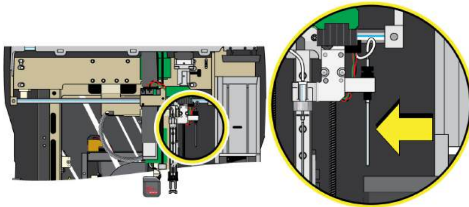
Figure 1.20 Dispense Probe - DxH Slidemaker Stainer II
