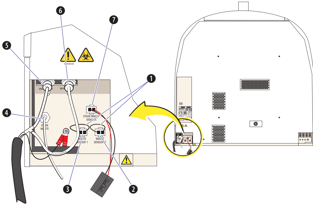
Figure F.8 Waste Connections Configured to Drain Directly into the Laboratory Drain
