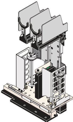
Figure 1.26 Basket Elevators
