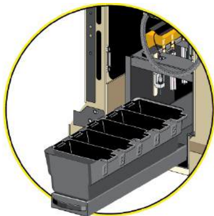
Figure 1.28 Stain Drawer
