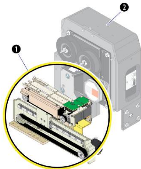
Figure 1.24 Print Shuttle
