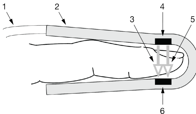
Figure 25 How a Pulse Oximeter Works
